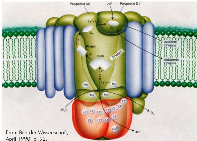
Photosystem II
